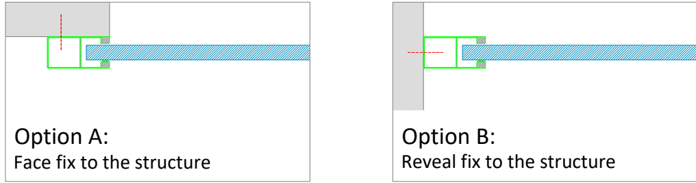
Guide fixing arrangements (scale 1:10)
