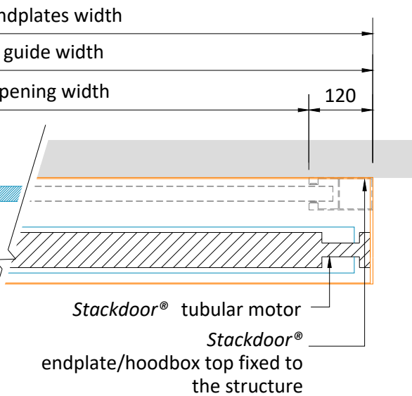
Plan Through: A-A (scale 1:10)
