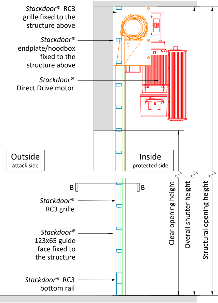
Section (when fully closed) (scale 1:10)
