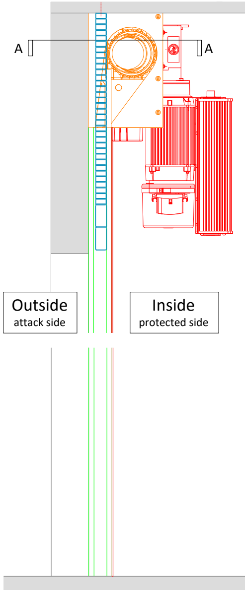
Section (when fully opened) (scale 1:10)
