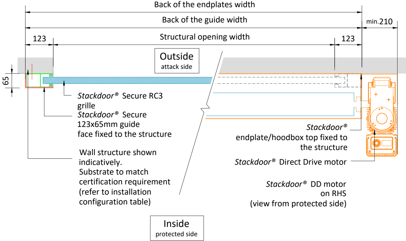
Plan Through: B-B (scale 1:10)
