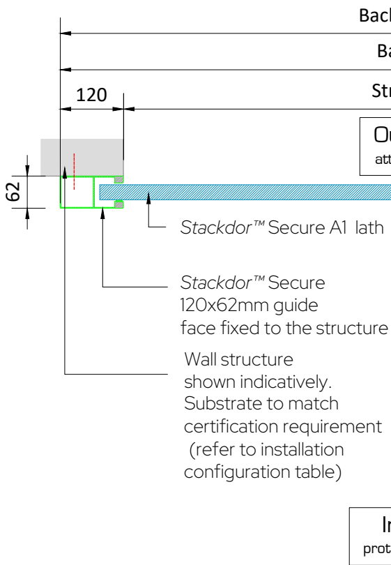
Plan Through: B-B (scale 1:10)
