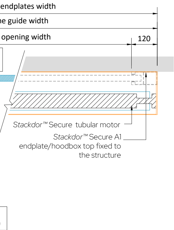
Plan Through: A-A (scale 1:10)
