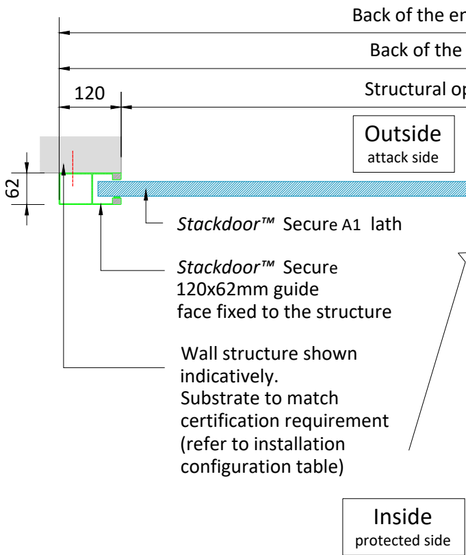
Plan Through: B-B (scale 1:10)
